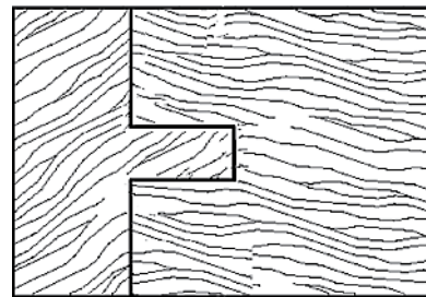
1 3 / 8 " Interior using one spacer & the 1/4" groover.
