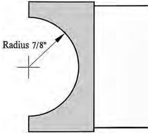
7/8" Radius Concave Half Round Edge Cutters
