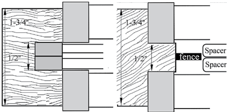
1 3 / 4 " Exterior Profile using 2 spacers & the 9/32" & 1/4" groovers.
